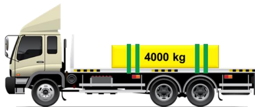
Not against headboard: twice the weight of the load (8000 kg) restraint
