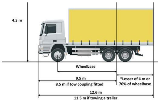
Exceeding legal vehicle dimensions
