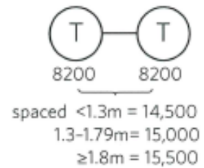
Exceeding group axle weight limits
