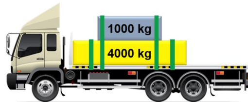
Heavy load low, light load high Keep the CoG as low as possible
